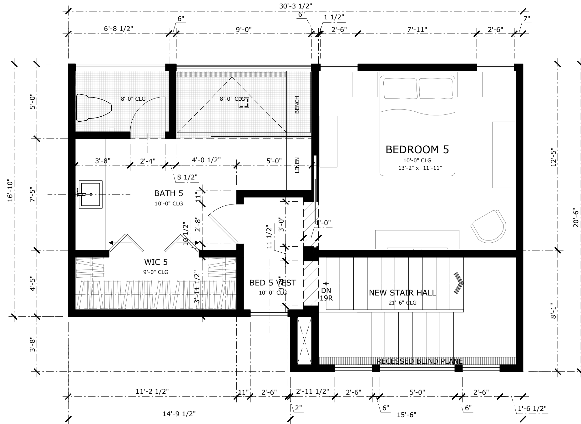
optional 2nd floor bedroom version 3
